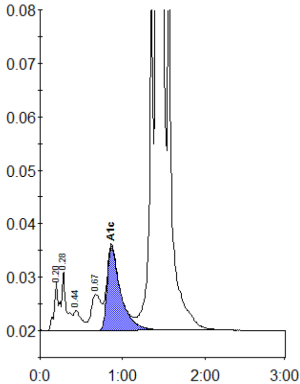
Peak table - ID: 10575644
